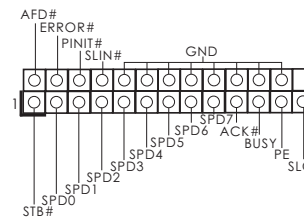
23 : 3-Pin Chassis FAN Connector (+12V)
