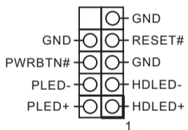
20 : System Panel Header
