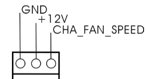
39 : 3-Pin Chassis FAN Connector (+12V)
