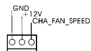
39 : 3-Pin Chassis FAN Connector (+12V)
