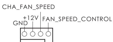
7 : 4-Pin Chassis FAN Connector (+12V)
